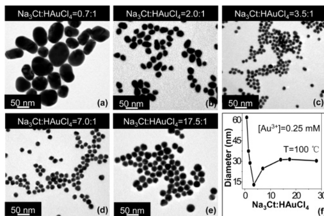
Figure 1. TEM images (a–e) and summary (f) of the average sizes of gold nanocrystals synthesized using different \text{Na}_3\text{Ct}/\text{HAuCl}_4 precursor ratios as labeled in each image. All nanocrystals were grown in boiling water using an initial \text{HAuCl}_4 concentration of 0.25 mM.
