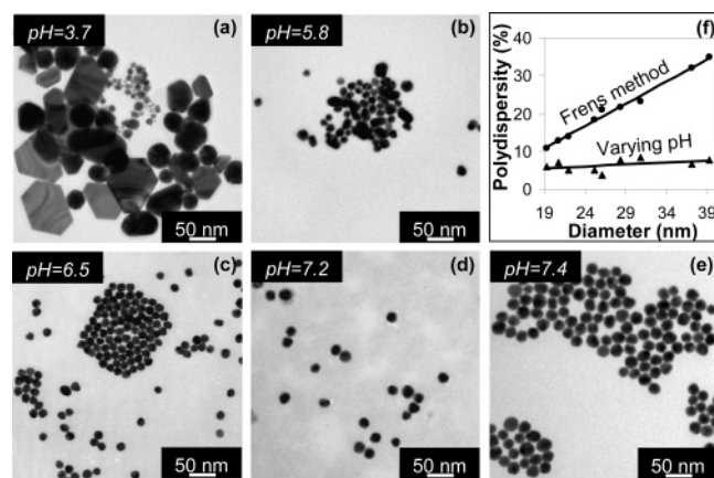
Figure 10. TEM images (a–e) of gold nanocrystals synthesized by varying the pH but with fixed initial Au(III) and Na 3 Ct concentrations. (f) Size distribution comparison between the Frens method and the strategy by varying pH with pH \geq 6.5 (see detail in text).
