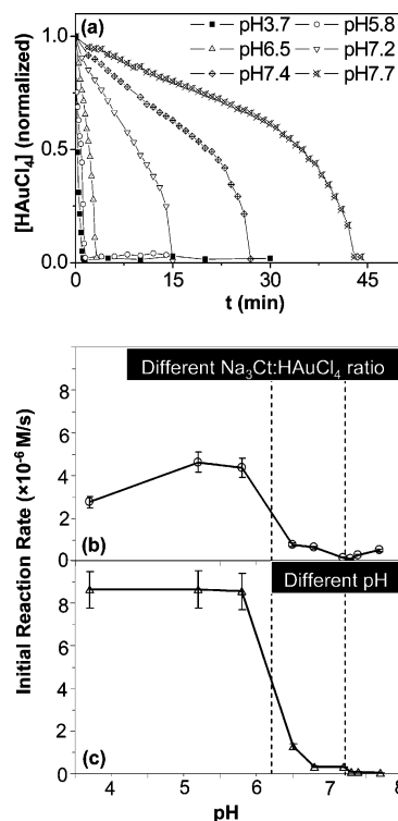
Figure 9. (a) Temporal evolution of Au(III) concentration of the reactions with variable pH at fixed initial Au(III) and \text{Na}_3\text{Ct} concentrations. (b) Initial reaction rates of Au(III) ion reduction determined for the reactions with variable \text{Na}_3\text{Ct}/\text{HAuCl}_4 ratios. (c) Initial reaction rates of Au(III) ion reduction determined for the reactions with a variable pH but a fixed \text{Na}_3\text{Ct}/\text{HAuCl}_4 ratio.
